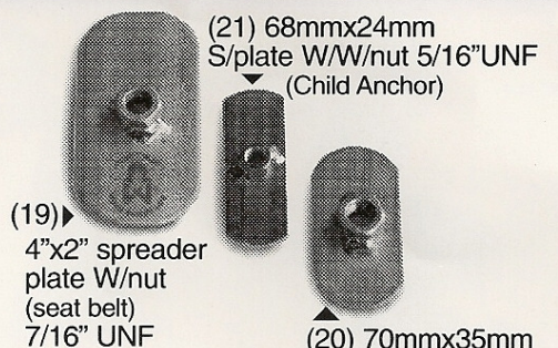
▶(20) 70mmx35mm S/plate W/W/nut 7/16"UNF Crab type
